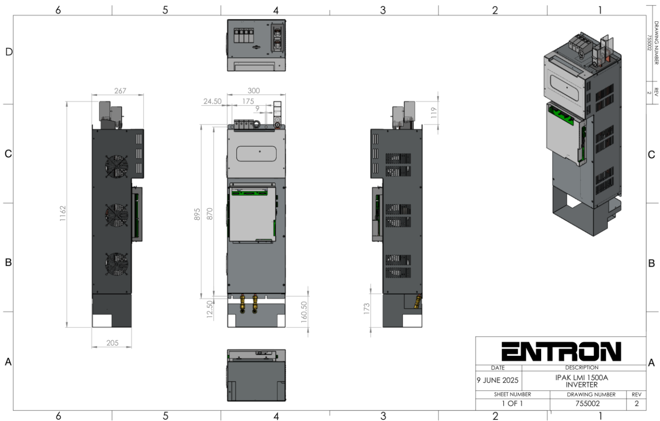
Outline Drawings – Inverter Modules (2 modules used per Inverter):
