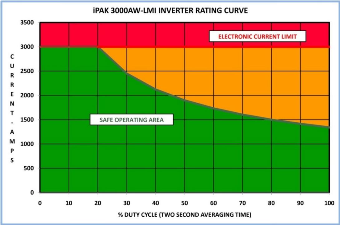
Rating Curve:
